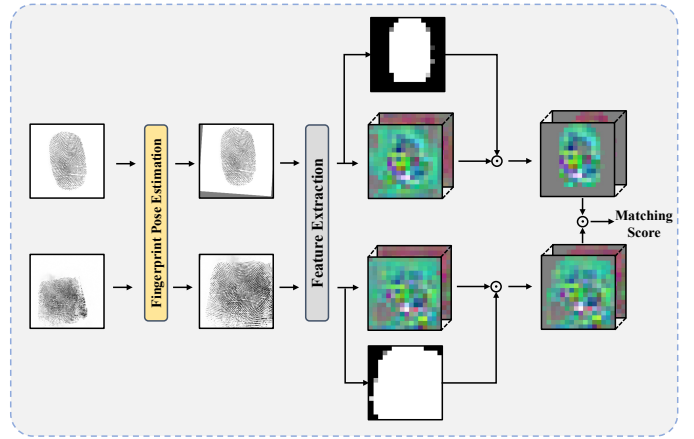
Fig. 2. Overview of fingerprint matching using the proposed FDD. First, fingerprint pose alignment is performed according to Duan et al. [22], followed by the extraction of fixed-length dense descriptors with the descriptor extraction network, which are then used for matching.
