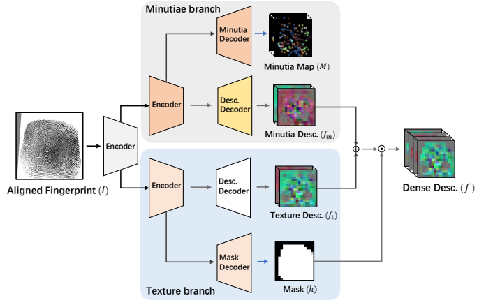
Fig. 3. The overall network architecture of FDD consists of the minutiae branch and the texture branch, which extract minutia maps and masks, respectively, along with their corresponding descriptors. “Desc.” is an abbreviation for “Descriptor”.
